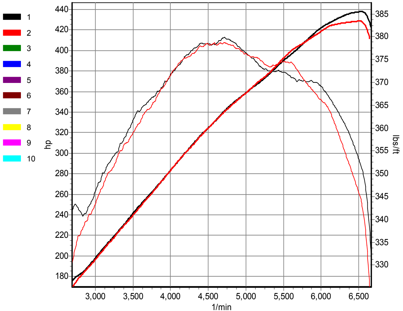
P-max Engine Power (corr.) / Speed / Torque (corr.)
